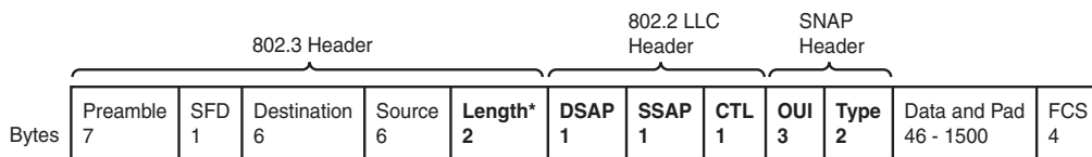
Figure 3-15 802.2 SNAP Headers
