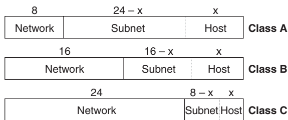
Figure 5-7 Address Formats When Subnetting Is Used (Classful)
