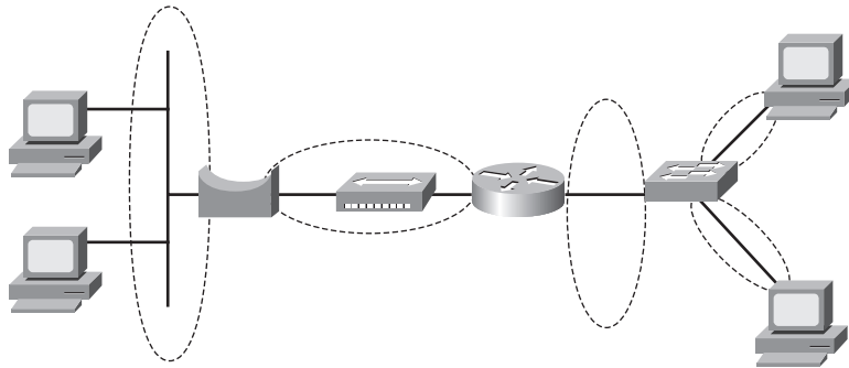
Figure 7-8 Collision Domains
